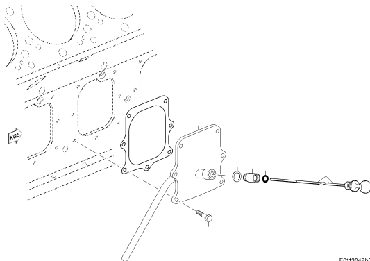
OIL DIPSTICK LEFT 010.00003
